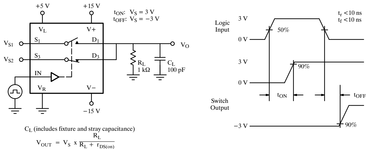
Figure 2. Switching Time
